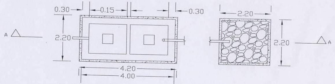
PLAN - SEPTIC TANK AND SOAK PIT
